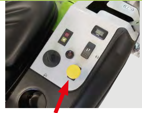
Electromagnetic clutch for blade engagement.
